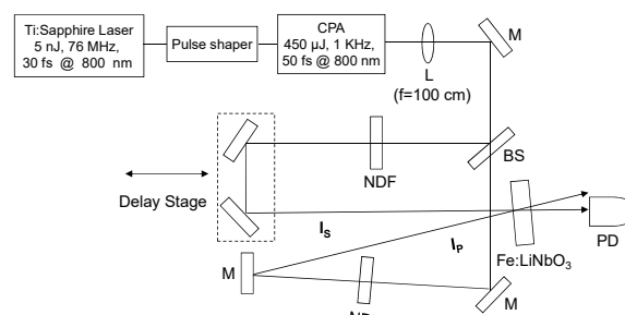
Fig. 1. Experimental setup.
